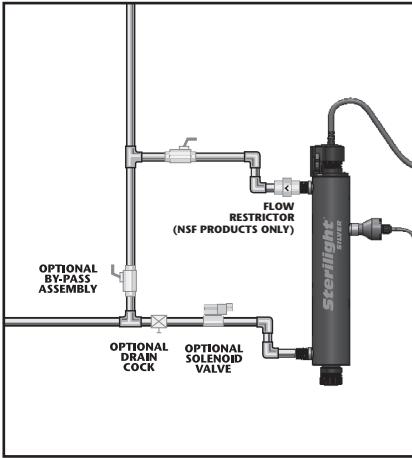
SOLENOID INSTALLATION
